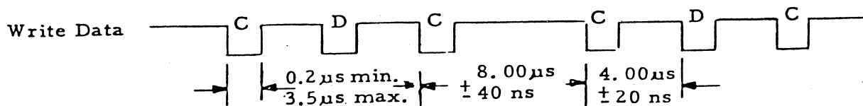
Figure 6 Write Data Timing
