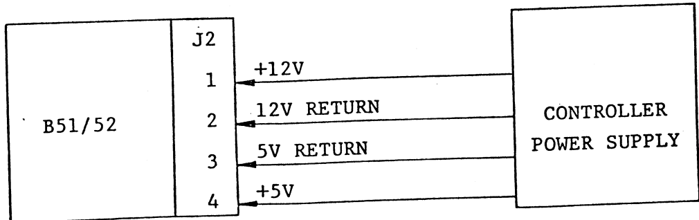
Figure 12 Interface Signals - B51/52
