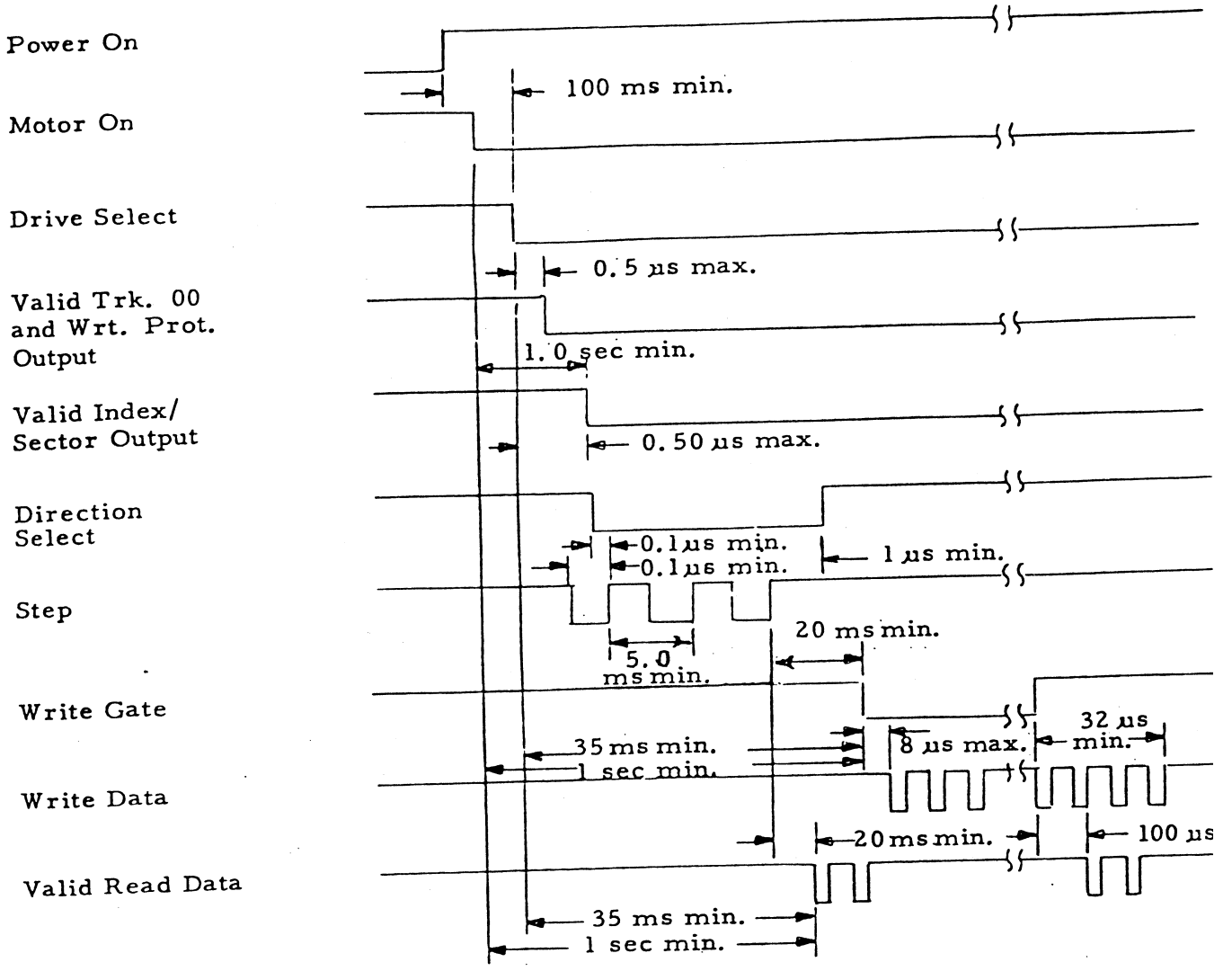
Figure 7 General Control and Data Timing Requirements
