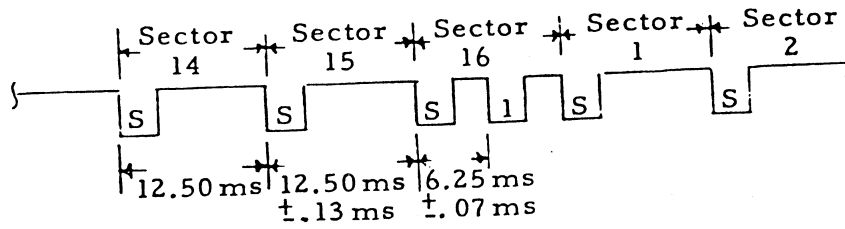
Figure 9 Index Sector Timing (Hard Sector)
