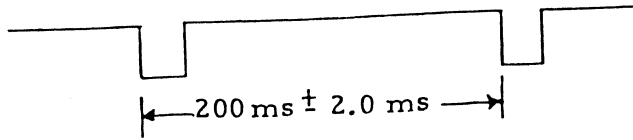
Figure 8 Index Sector Timing (Soft Sector)
